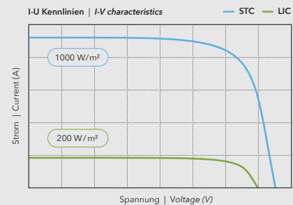
I-U Kennlinien | I-V characteristics
